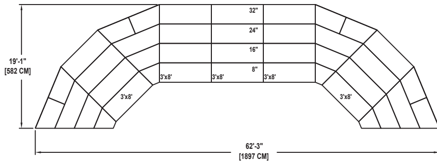
ARC SHAPE
