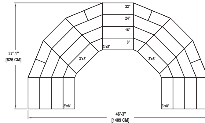
SEMICIRCLE SHAPE
