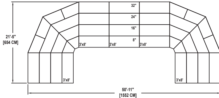
HORSESHOE SHAPE
